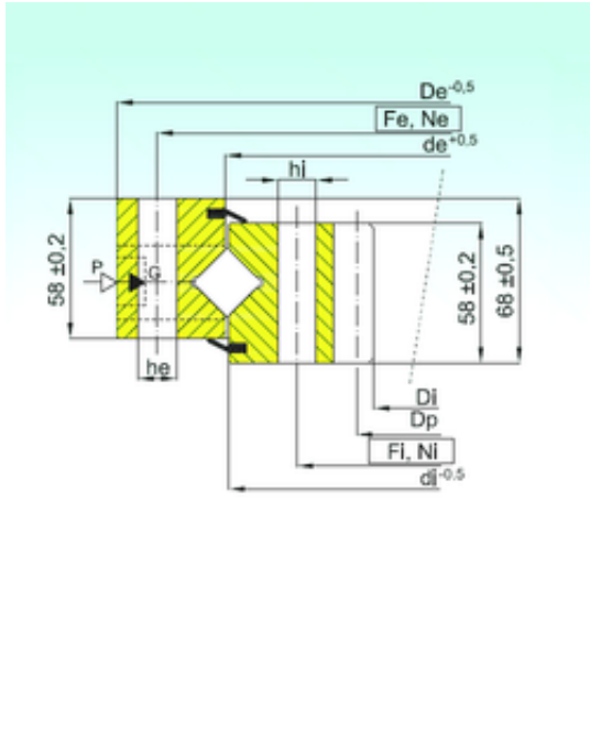
ZR1.20.1904.400-1SPPN Bearing 2D drawings and 3D CAD models
