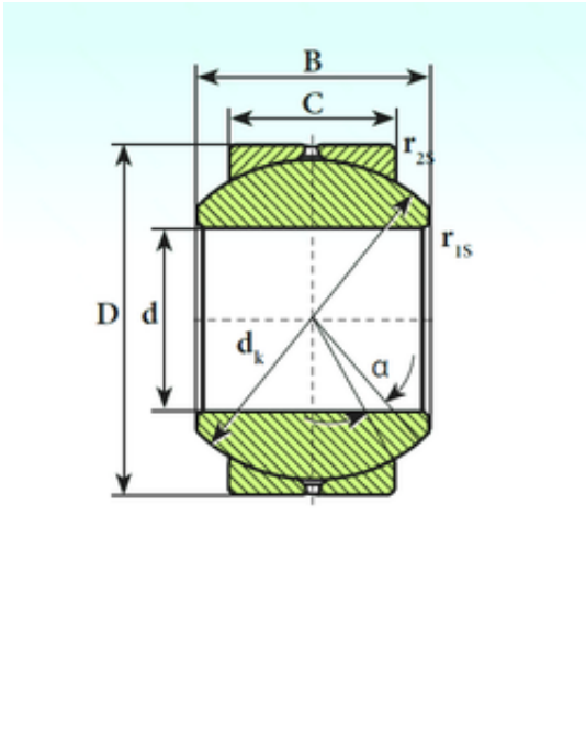
GE 20 SB Bearing 2D drawings and 3D CAD models
