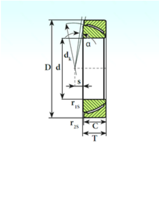
GAC 35 SP Bearing 2D drawings and 3D CAD models
