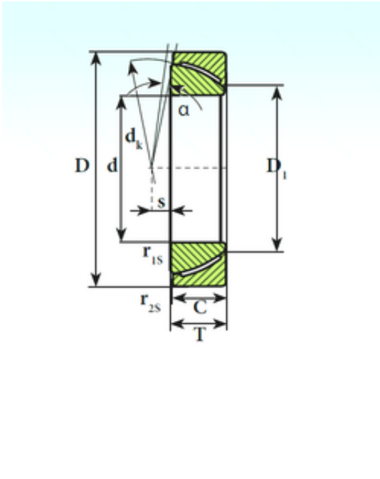
GAC 85 CP Bearing 2D drawings and 3D CAD models
